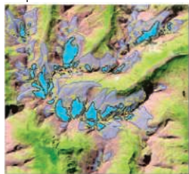
The extent of glaciers in the Rheinwald region (1850, blue line; 1973, yellow; 1999, black).
